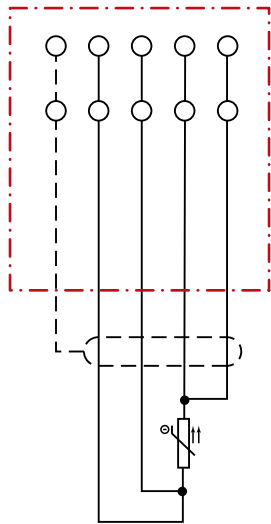
Connection of 1 PT100 4-wire
