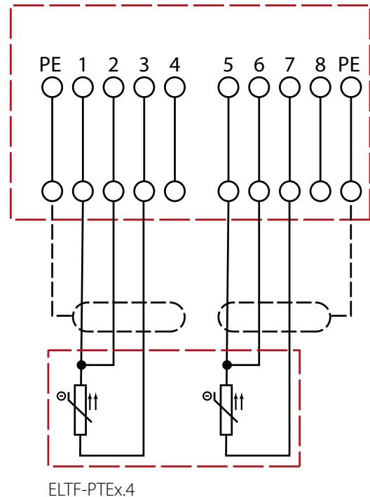
Connection of 1x double PT100
