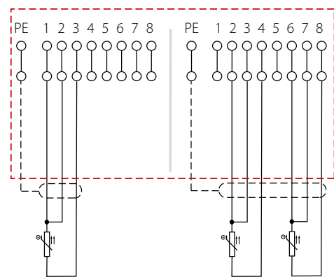
Connection of 1 or 2 Pt100
