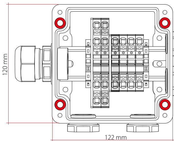
Star point ELK-MI-TWIN & star point 3 phases ELK-MI-SINGLE
