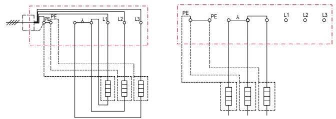
Star point ELK-MI-TWIN & star point 3 phases ELK-MI-SINGLE
