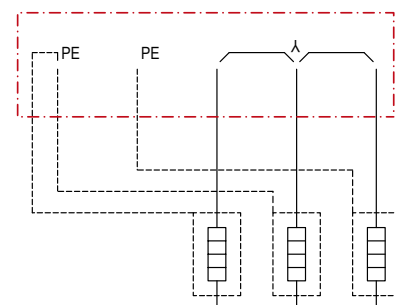
Star configuration
