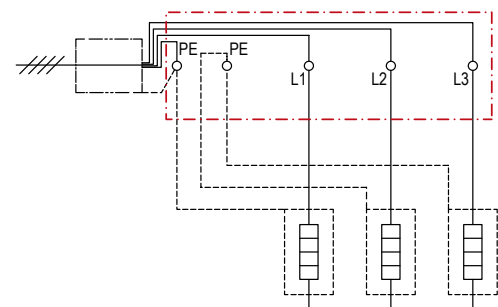
3 phases connected
